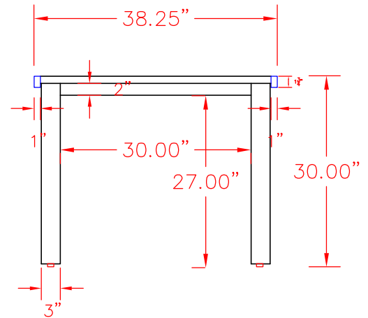
Budget Edge Wooden Legs
