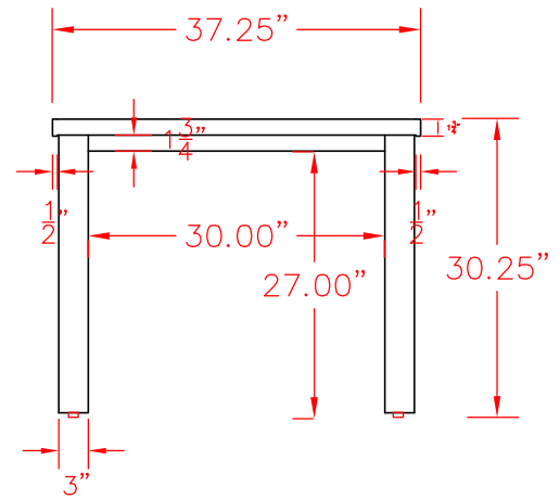
Budget Edge Wooden Legs
