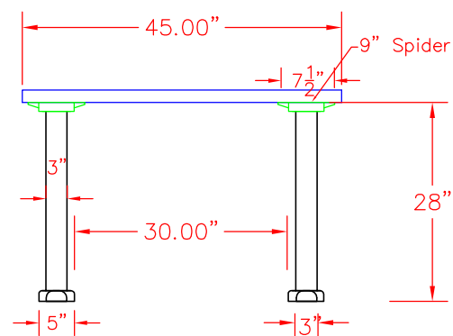
Eased Edge Metal T Bases
