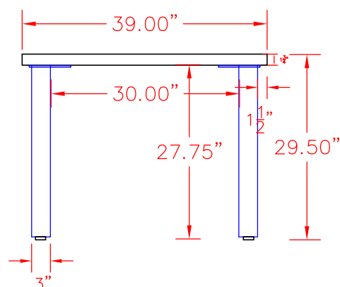
Budget Edge Metal Legs
