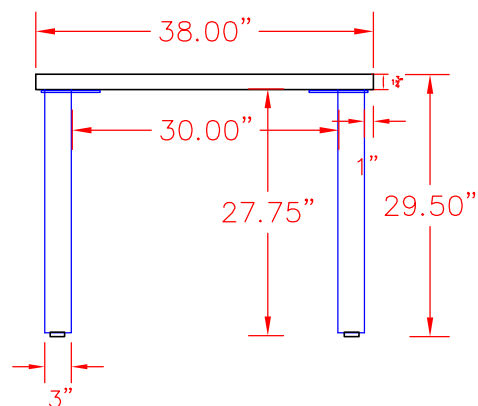
Eased Edge Metal Legs
