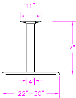
T FOOT BASE
