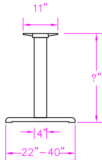
X FOOT BASE
