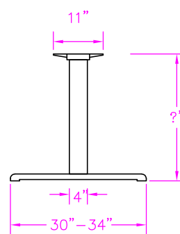
Extended X FOOT BASE
